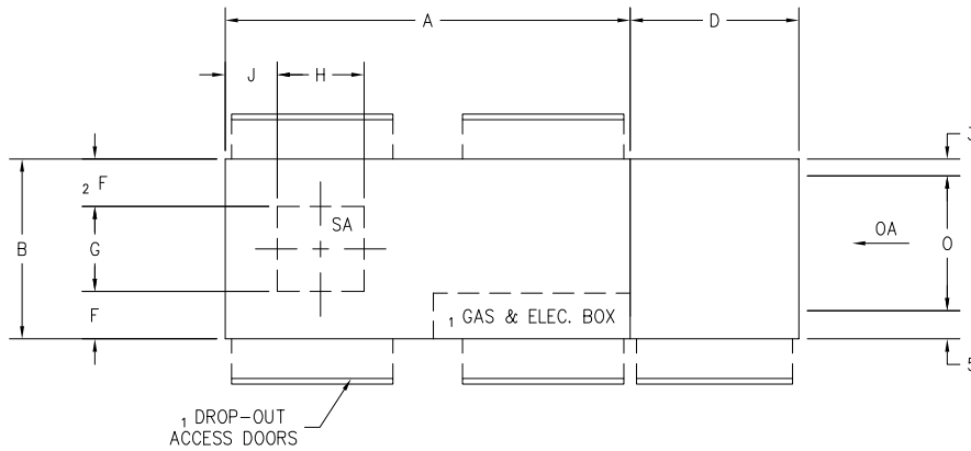
PLAN VIEW
