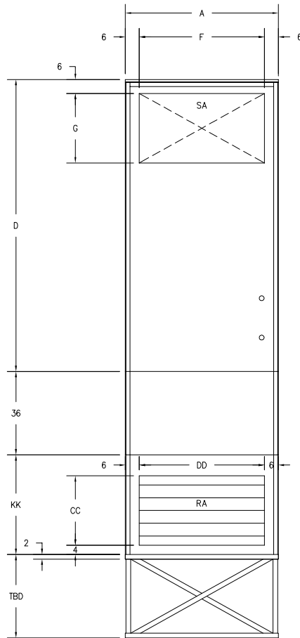
BOTTOM SIDE VIEW
