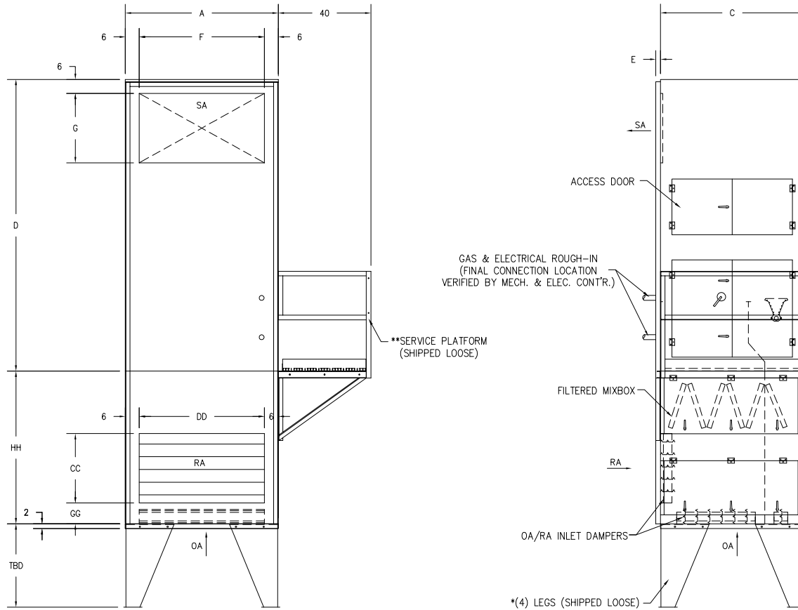
BOTTOM SIDE VIEW
