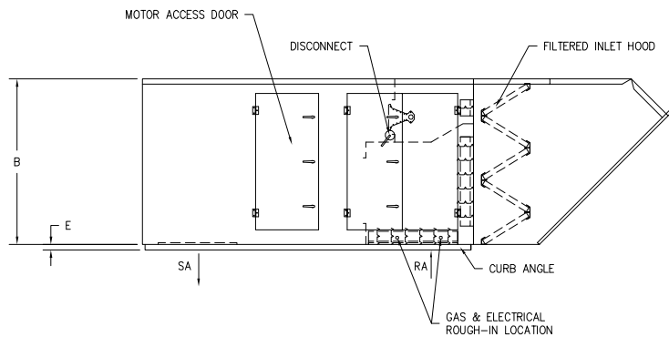
CONTROLS SIDE VIEW
