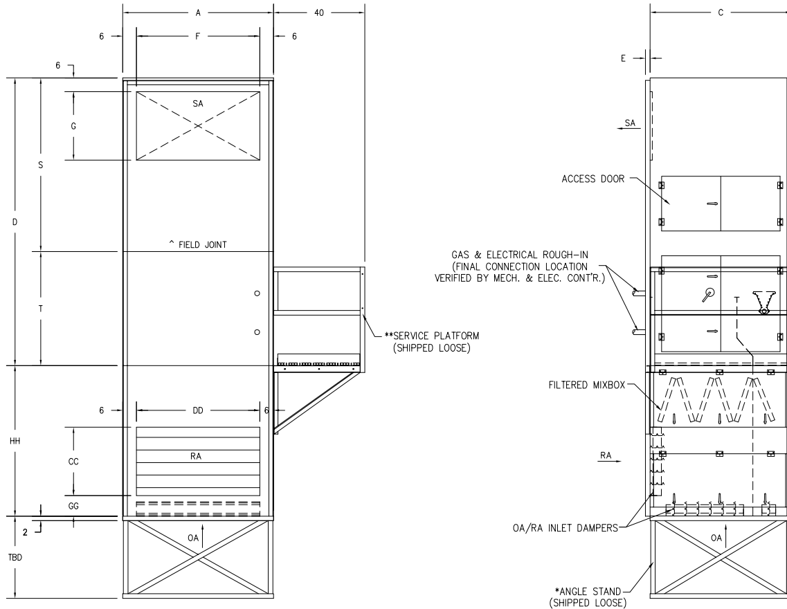
BOTTOM SIDE VIEW
