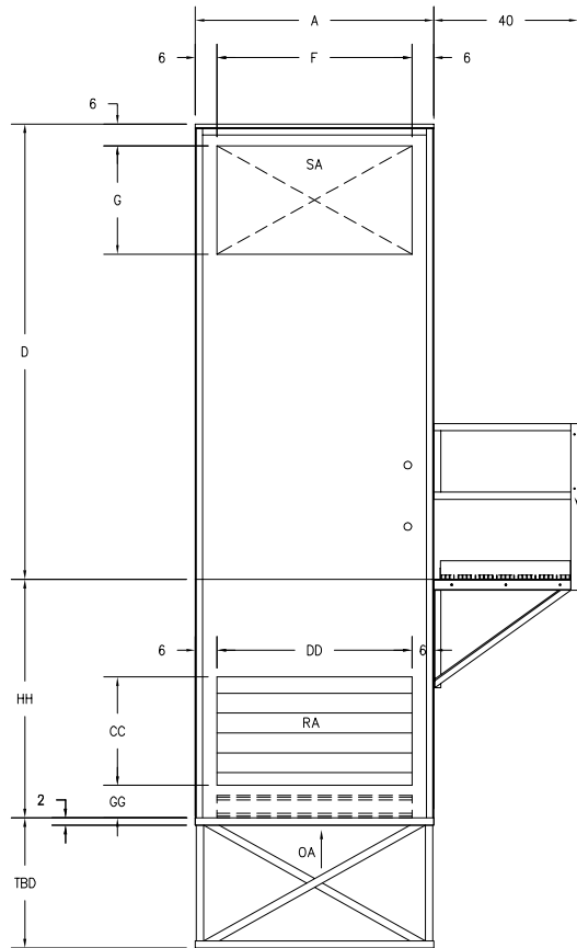
BOTTOM SIDE VIEW
