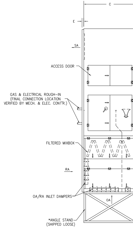
CONTROLS SIDE VIEW
