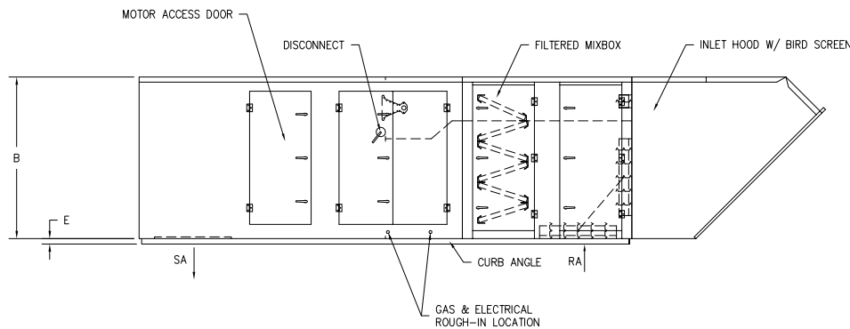
CONTROLS SIDE VIEW
