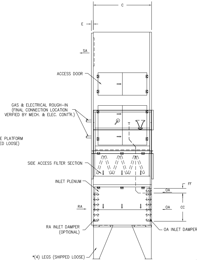
CONTROLS SIDE VIEW
