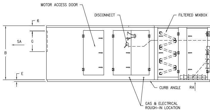
CONTROLS SIDE VIEW
