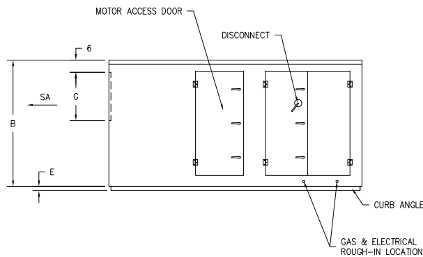
CONTROLS SIDE VIEW
