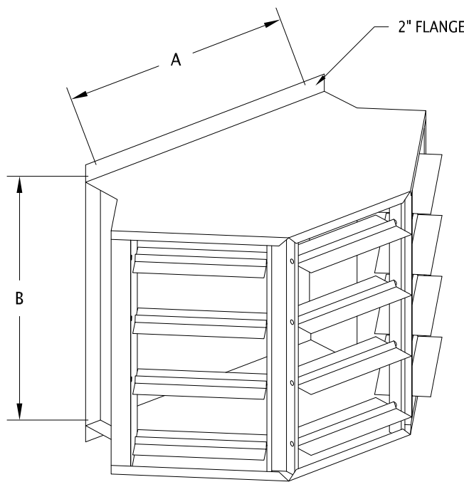
ISOMETRIC VIEW
