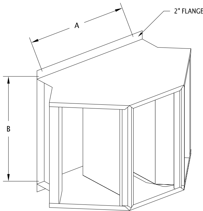
ISOMETRIC VIEW
