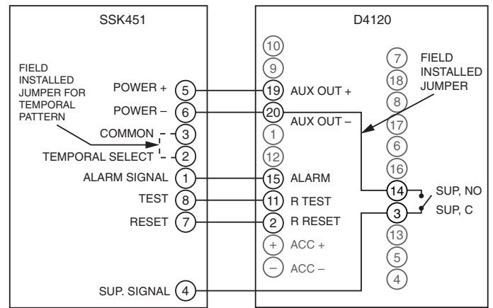
Figure 12. Wiring diagram for D4120 to SSK451:
