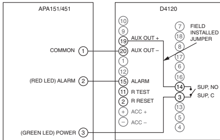
Figure 9. Wiring diagram for D4120 to APA151 or APA451:
