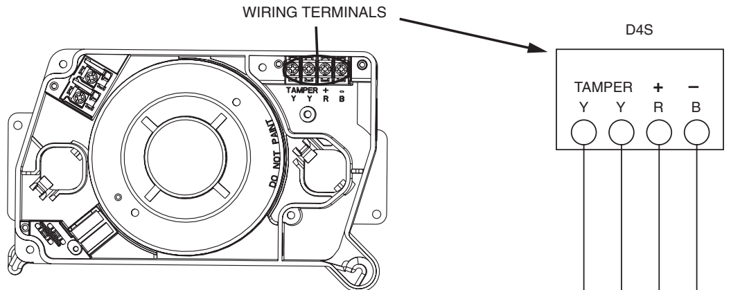
Figure 13. Optional sensor 2 configuration and wiring:
