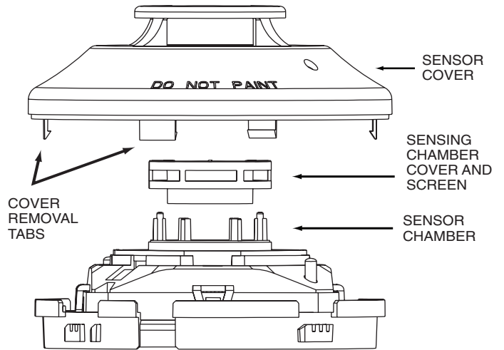
Figure 10. Detector sensor exploded view:
