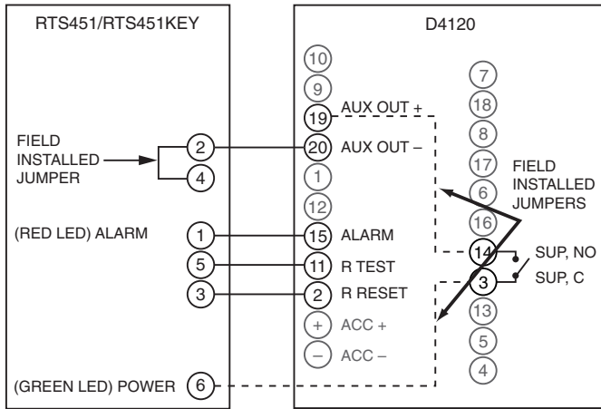
Figure 11. Wiring diagram for D4120 to RTS451/RTS451KEY:
