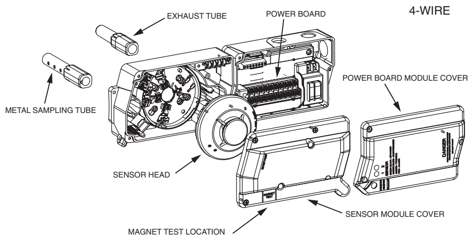
[1] Figure 1. Exploded View of Duct Smoke Detector Components:
