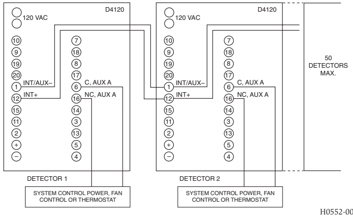
Figure 6. Multiple Fan Shutdown (interconnection of D4120's):
