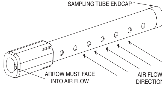
Figure 3. Air duct detector sampling tube:
