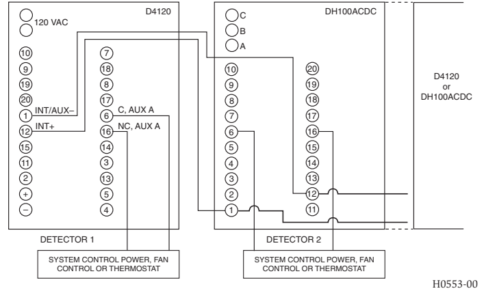
Figure 7. Multiple Fan Shutdown (interconnection of D4120 to DH100ACDC):
