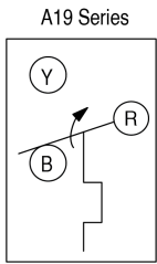
Figure 1: A19 Series terminal arrangement for Single-Pole, Double-Throw (SPDT)
