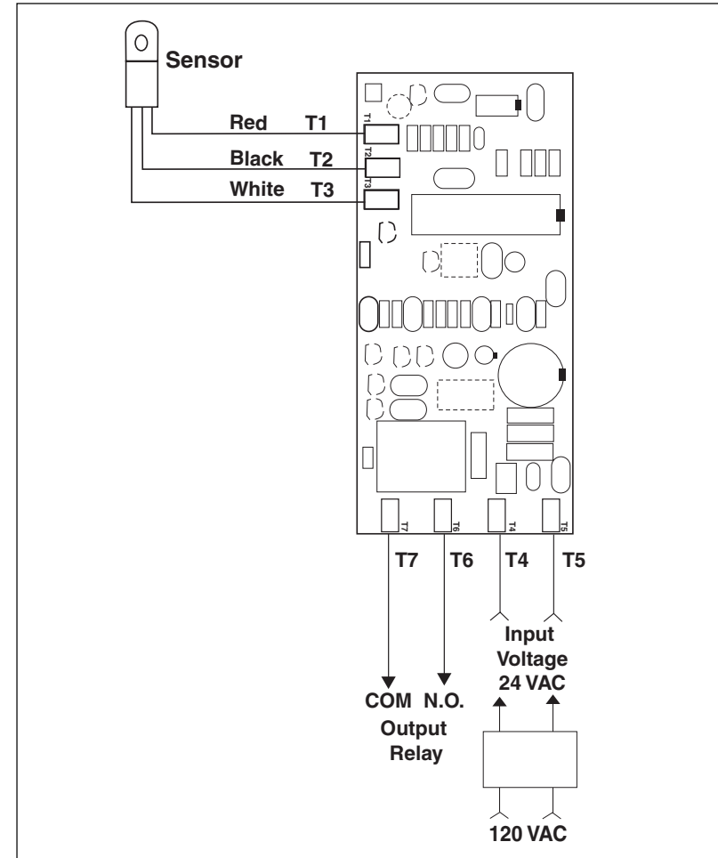
Figure 2- Wiring Diagram
